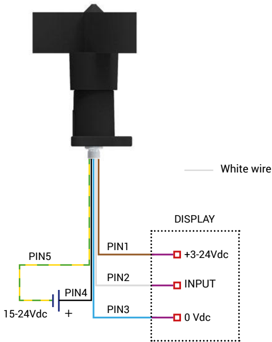
Blocks diagram
