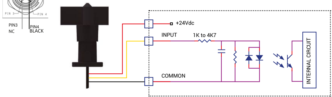
3-wire connection to a PLC
